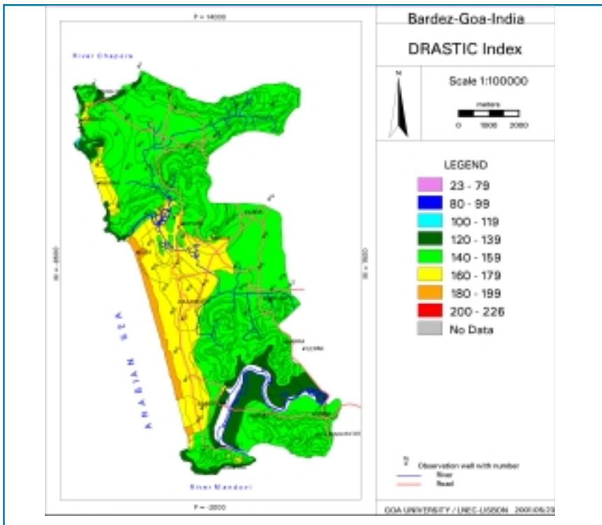
Figure 8 Mapping aquifer vulnerability using DRASTIC
