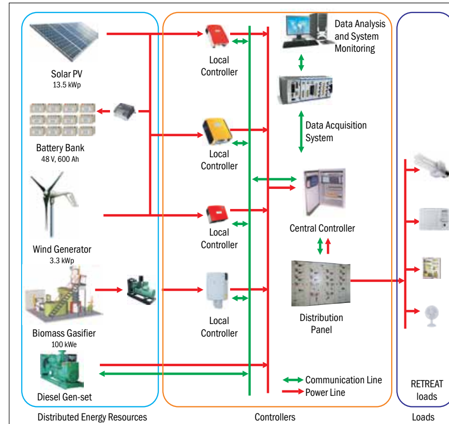
Schematic of Smart Mini-Grid at TERI Gram
