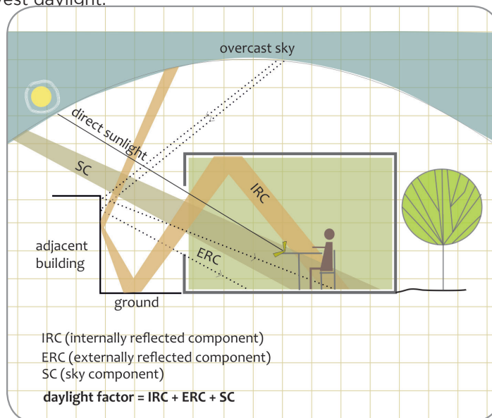
Figure 45 Daylighting as a passive design strategy
